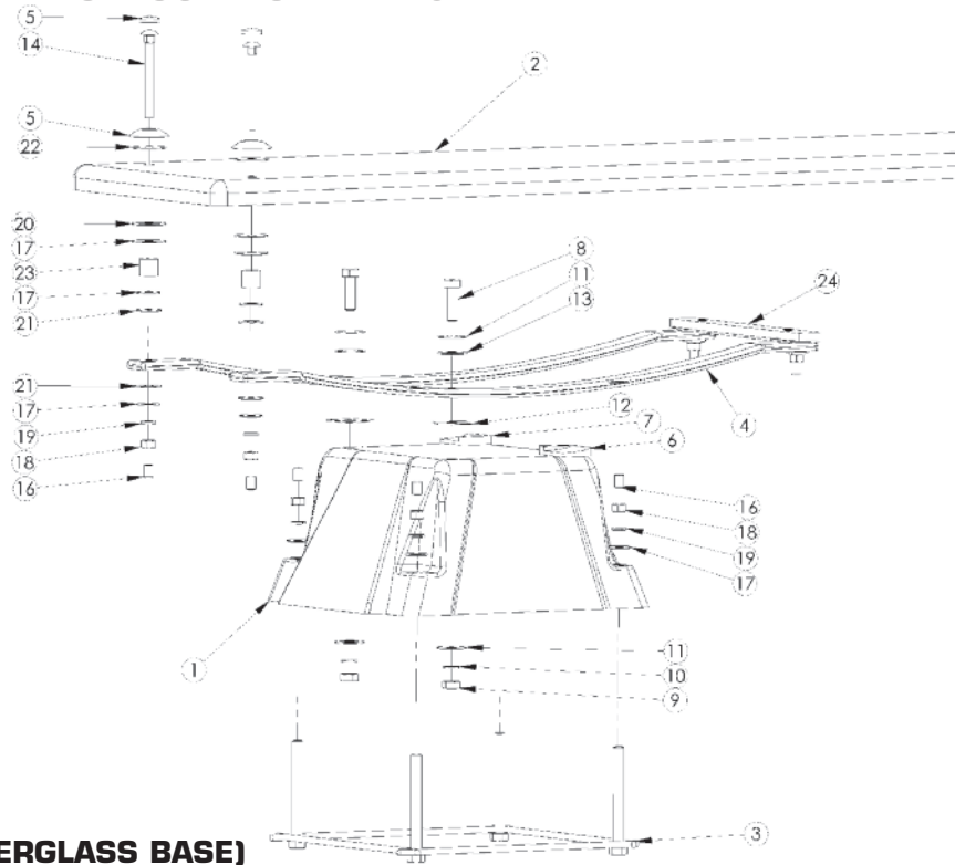
FIG. F – TECHNI-SPRING FIBERGLASS BASE EXPLODED VIEW
